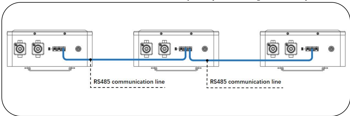
Figure 18 Sample of Connection the RS485 Communication Cable
