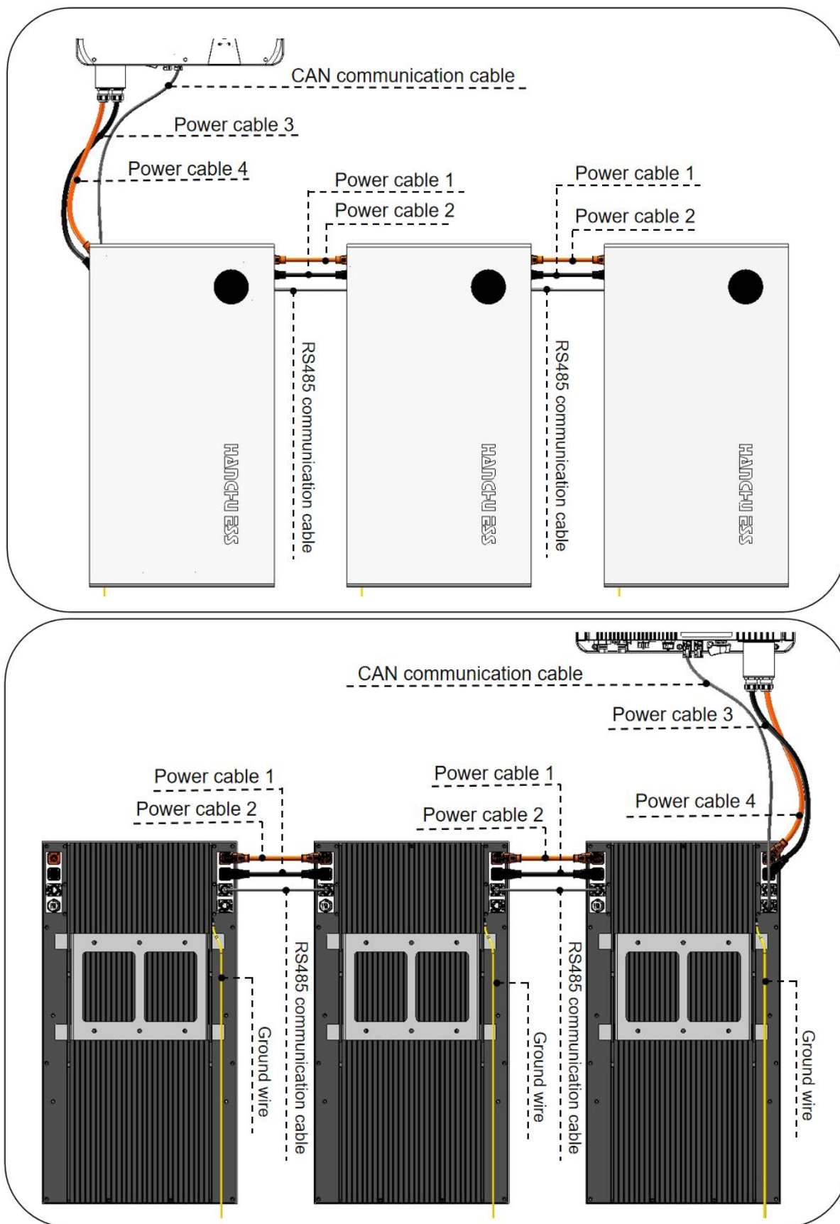
Figure 12 System General Wiring Diagram
