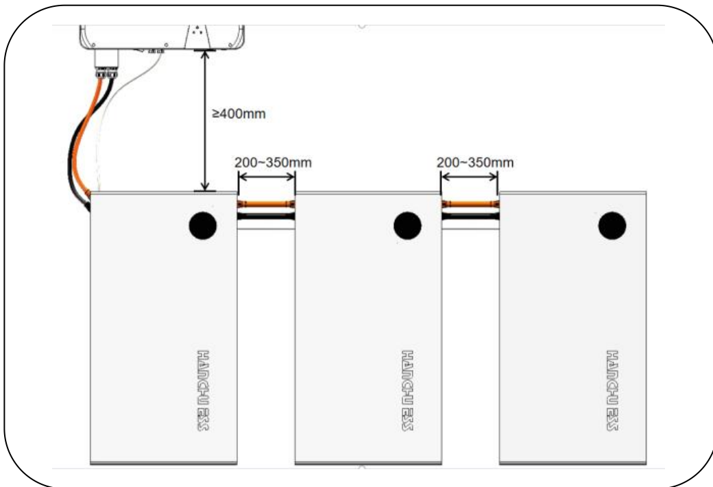
Figure 8 Sample of Step 3 for Floor Installation
