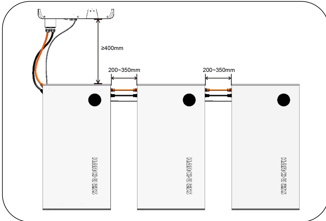
Figure 11 Sample of Step 3 for Wall Installation
